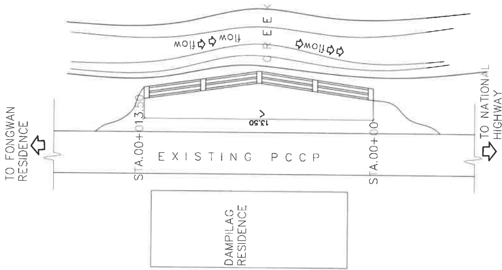
SITE DEVELOPMENT PLAN
