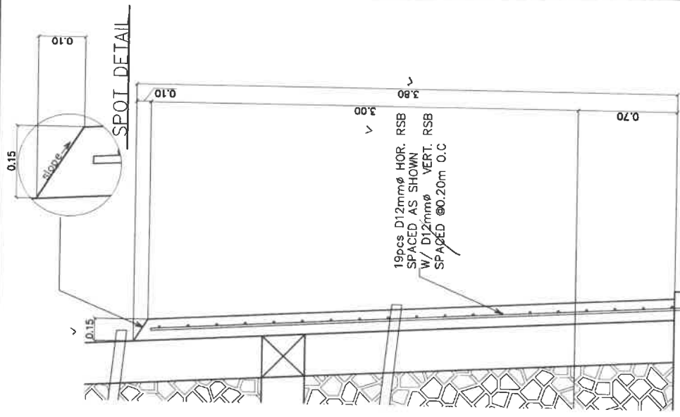
RC ARMOR DETAIL SCALE 1:25
