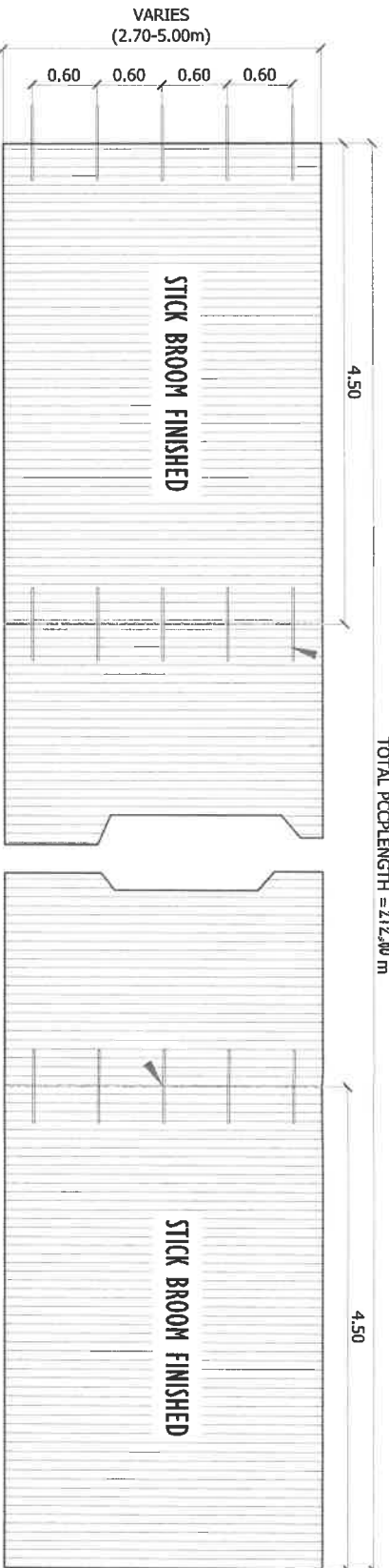
PCCP PLAN (STA 03+000 - 03+212) SCALE N/DTS
