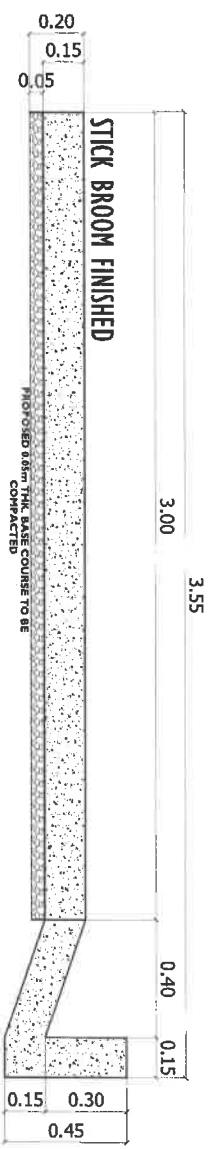
EXPANSION JOINT @ EVERY 4.50m WITH 6mm x 50mm HOT ASPHALT FILLER
