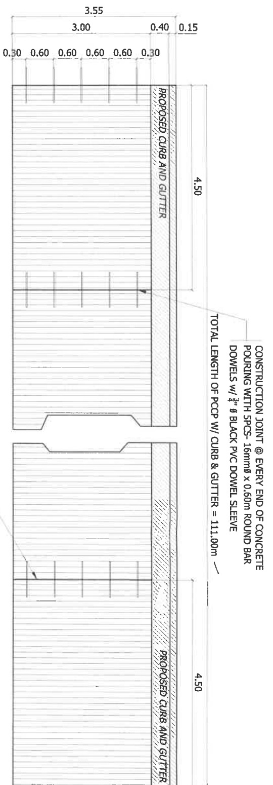
PCCP W/ CURB & GUTTER PLAN (STA 03+500 - 03+611) SCALE NDT'S
