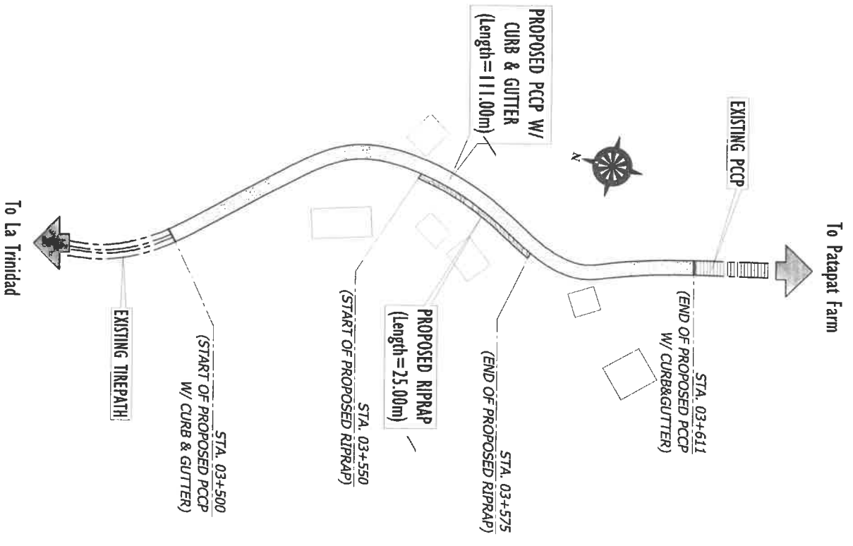
DEVELOPMENT PLAN SCALE NDT'S
