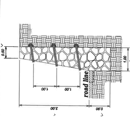
PROPOSED RW-2 SECTION
