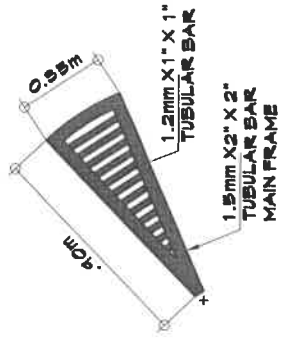
STAIR THREAD DETAIL SCALE 1:30M
