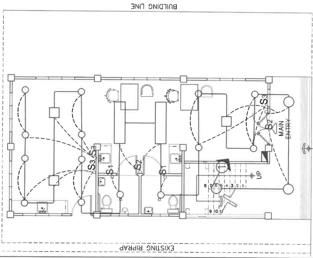
E4 LIGHTING LAYOUT FIRST FLOOR
