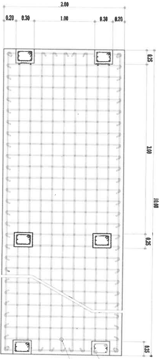
AVERAGE CROSS-SECTION (LENGTH = 10.00 m.)
