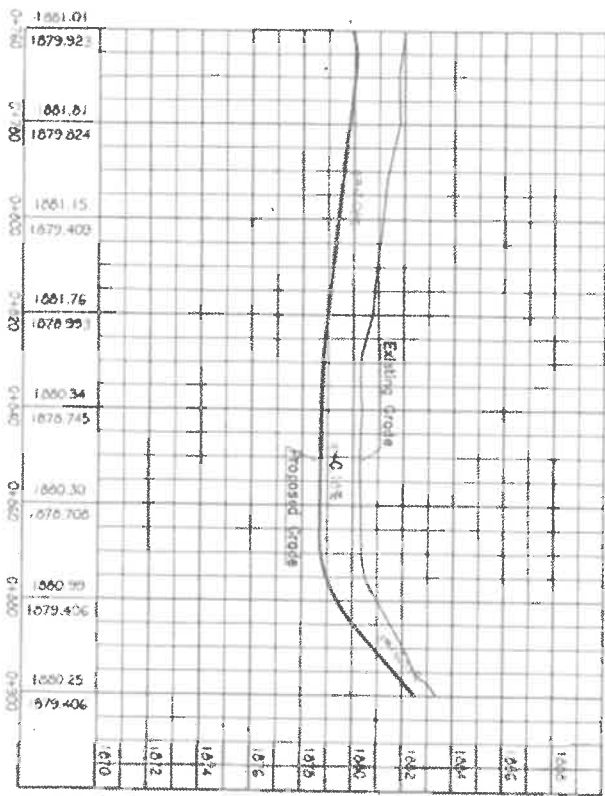
PROFILE OF 0+760 TO 0+900 SCALE: Horizontal 1:1000 Vertical 1:200
