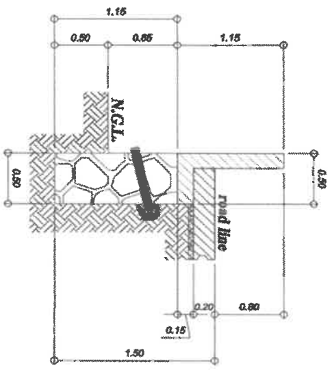
RW-4 SECTION SCALE ----- HD15
