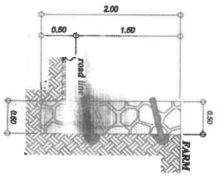
PROPOSED RETAINING WALL-3 ELEVATION @ STA.00+105.00 TO STA.00+115.00
