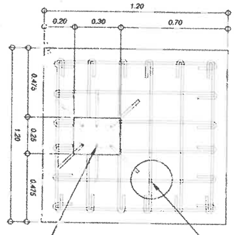
ISOLATED FOOTING-2 PLAN(2UNITS) SCALE ..... NDTS
