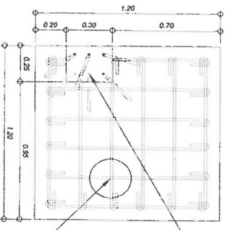
ISOLATED FOOTING-1 PLAN(2UNITS) SCALE ..... NDTS
