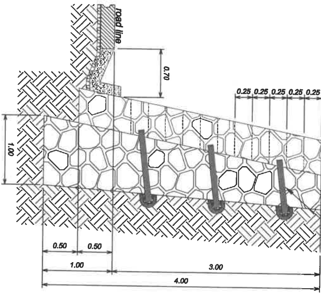
RW-2 SECTION @ STA.00+041.80(after) TO STA.00+060.00(before)
