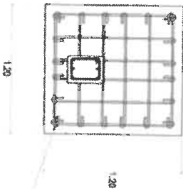
TYPICAL FOOTING DETAILS
