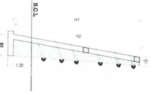
TYPICAL RETAINING WALL SECTION DETAILS ("A" TO "O") SCALE
