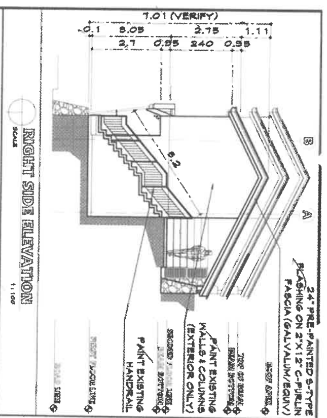
RIGHT SIDE ELEVATION SCALE 1:100
