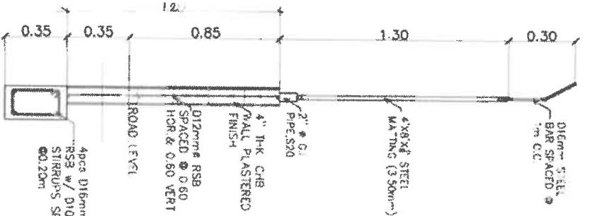
FENCE WALL ELEVATION SCALE 1:70
