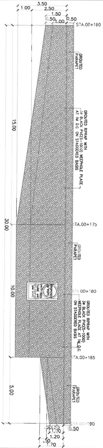
GROUTED RIPRAP ELEVATION SCALE 1:85
