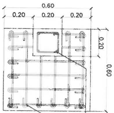
FOOTING DETAIL SCALE 1:10
