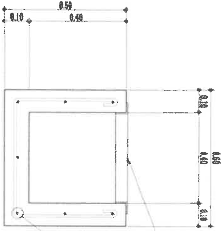
PROPOSED CANAL-1 WITH STEEL GRATING SECTION DETAIL SCALE NOTES
