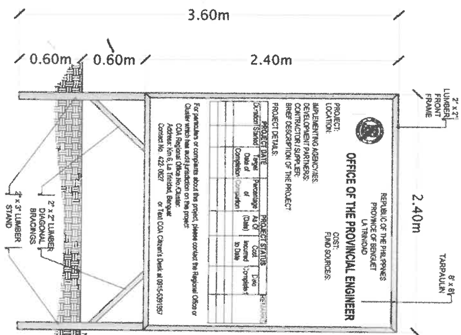
FRONT ELEVATION
