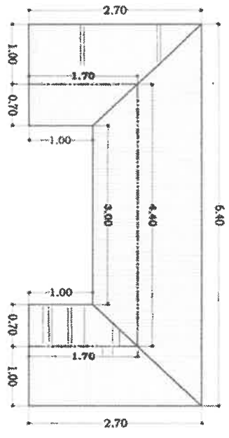
PROPOSED WINGWALL PLAN DETAILS
